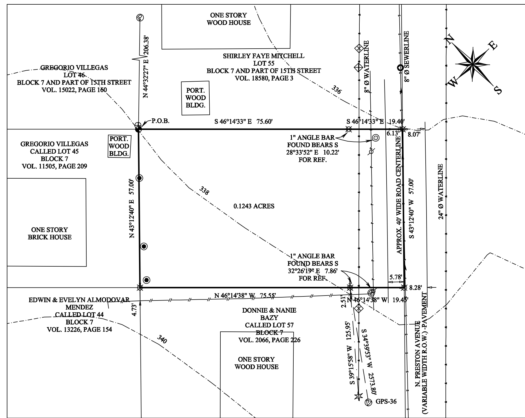
PRELIMINARY PLAN
